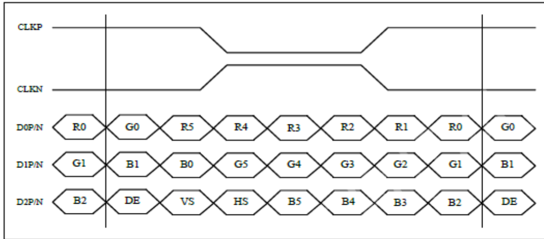
6-bit LVDS input (LVBIT=L, LVFMT=Don't care)
